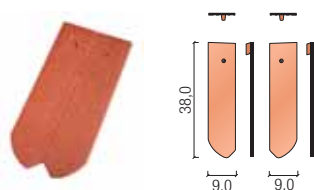
dachówka 3/4
